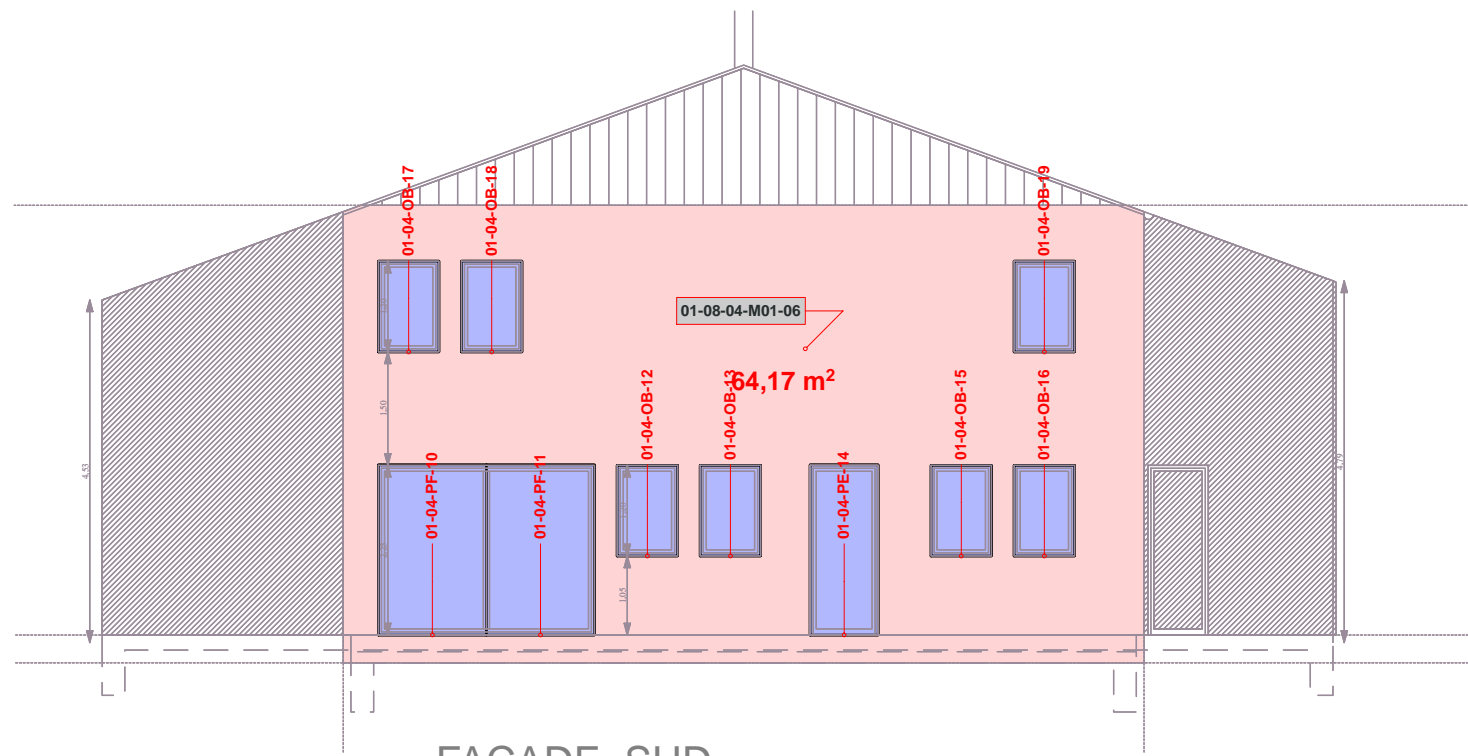
FACADE SUD
